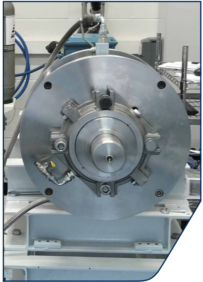
Dynamic test rig with 7.500" (190mm) RDSX™ installed
