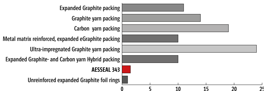
Weight loss after the exposure to temperature of 600 °C in stuffingbox
