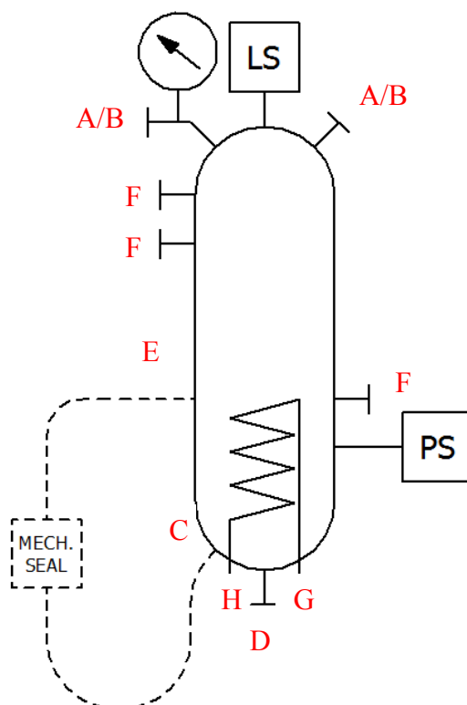
Fig.2 Plan 53A with Screwed connections
